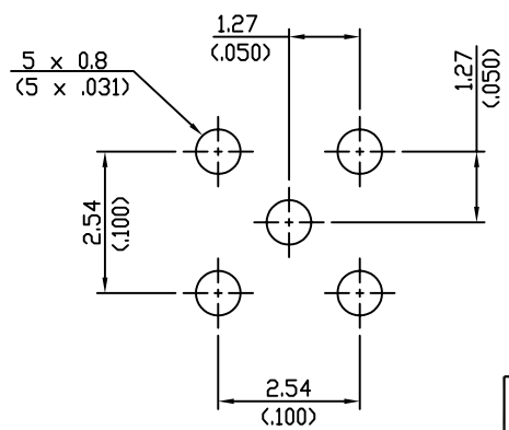
Mounting hole
